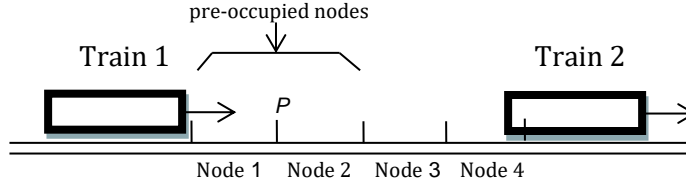
Figure 4. Dynamic headway model
