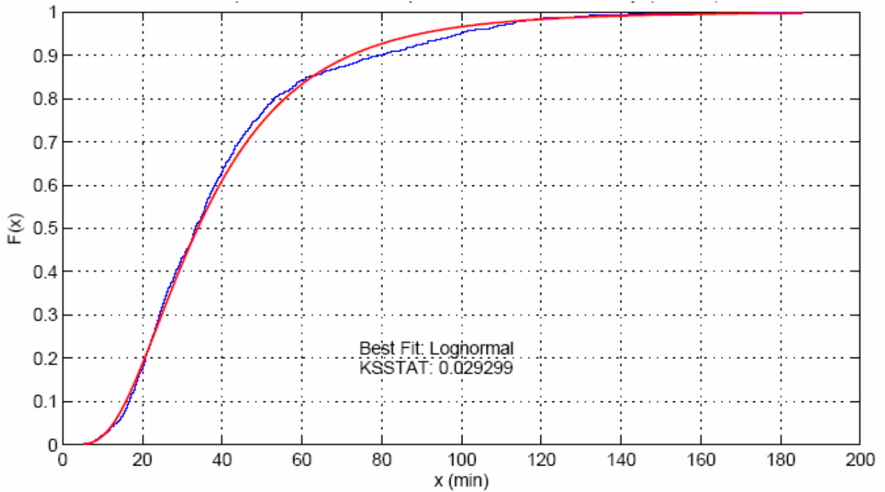
Figure 8: Empirical CDF of Turn Times for Bobtail and Main Entries on All Days.
