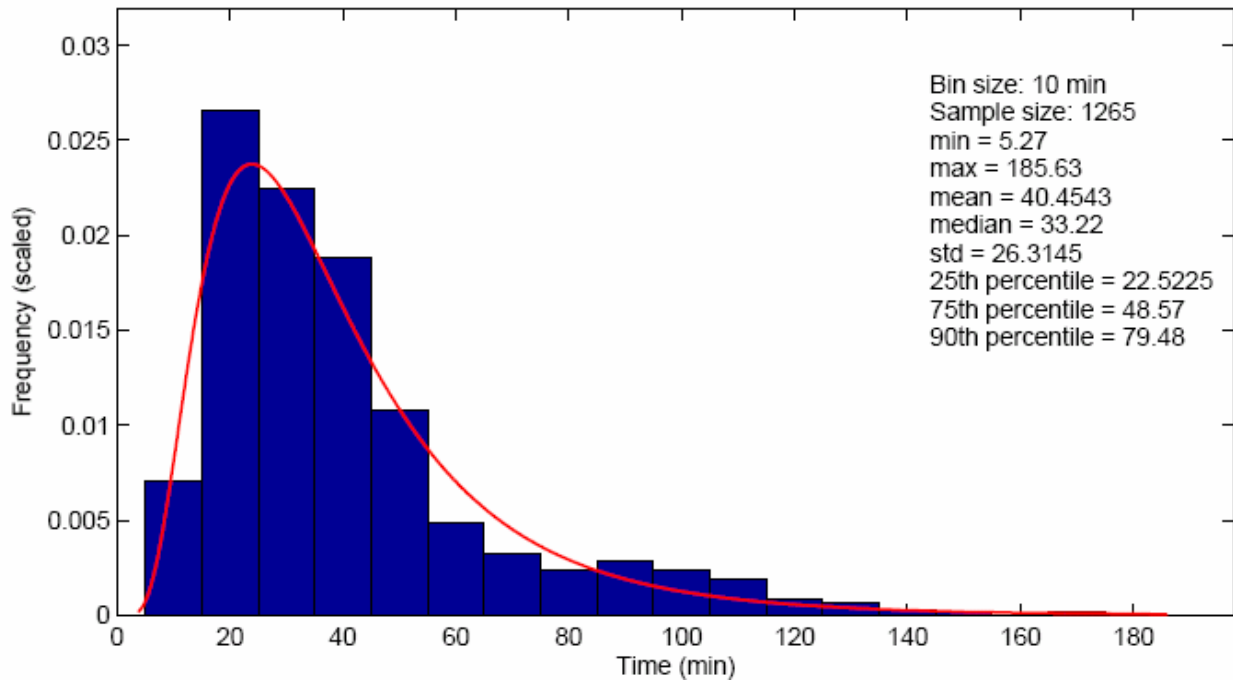
Figure 7: Distribution of Turn Times for Bobtail and Main Entries on All Days.
