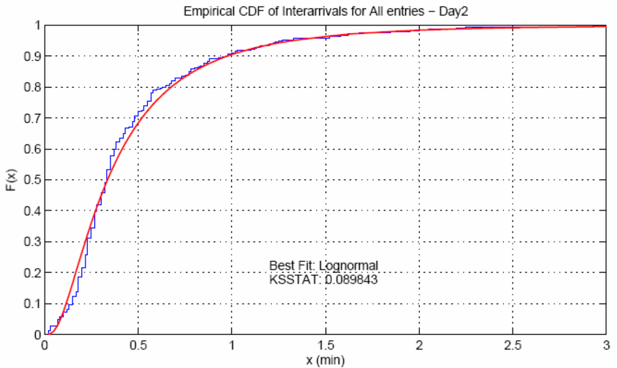
Figure 6: Empirical CDF of Interarrivals for Both Entries on Day 2
