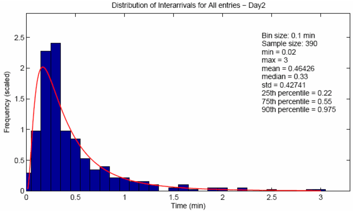
Figure 5: Distribution of Interarrivals to Both Entries on Day 2
