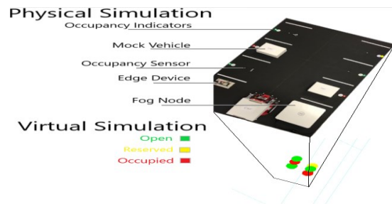
Figure 9: Hardware-in-the-loop and software simulation layout
