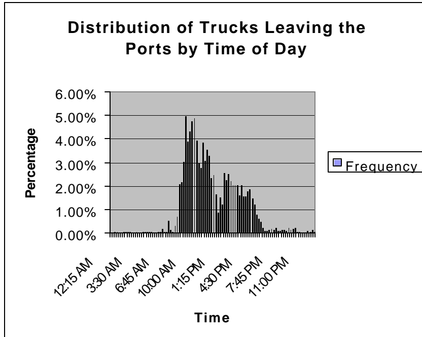
Figure 10. Distribution of Truck Trips Leaving the Ports by Time of Day
