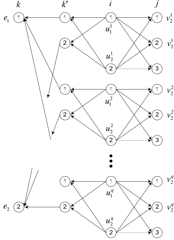
Figure 4: Multi-commodity substitution model, where m = 1 , n = 2 , and p = 1 .
