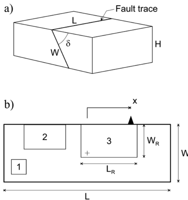
Fig. 1 (a) Model geometry. (b) The fault surface and three possible ruptures, only one of which (no. 3) affects the site (no. 1 does not break the surface and does not extend horizontally to the site; no. 2 breaks the surface but does not extend to the site).
